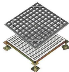
55% ventilation
